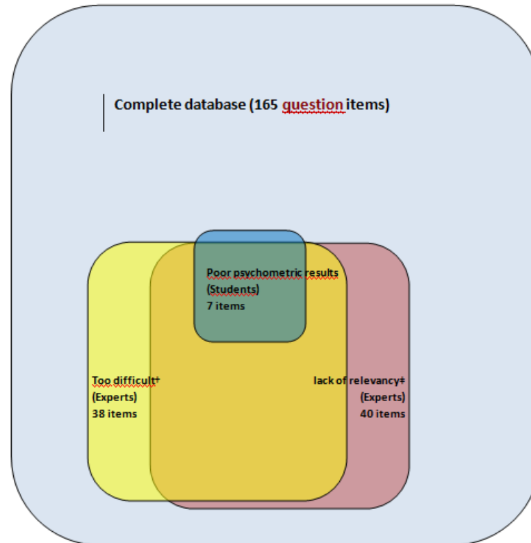
Figure 1: Ueeler diagram of items for revision ordered by selection criterion
